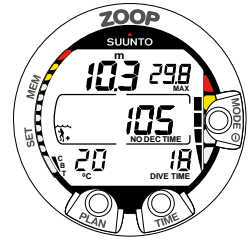
Fig. 3.11. Ascent Rate Indicator. Maximum allowed ascent rate. Four segments
