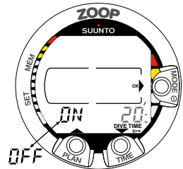
Fig. 4.19. Setting Dive Time Alarm. Press scroll buttons to change alarm on/off and to set dive time value.
