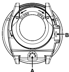
Fig 2.3. Depth sensor (A), water/data transfer contacts (B).
