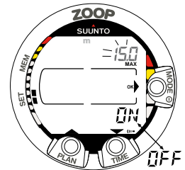
Fig. 4.20. Setting Maximum Depth Alarm. Press scroll buttons to change alarm on/off and to set maximum depth value.
